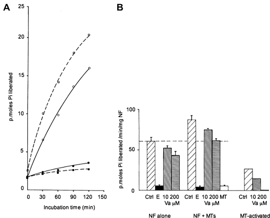
Fig. 3. Effect of microtubules and vanadate on the NF-bound ATPase activity. The ATPase activity of 0.25 mg/ml NFs was analyzed in buffer B + 6 mM \text{MgCl}_2 at 35 °C in the presence of 0.3 mM \gamma\text{-}^{32}\text{P} -ATP alone or in the presence of 1 mg/ml taxol-stabilized tubulin polymers. (A) Time course of ATPase of NFs (plain line, open circles) and NFs + MTs (dotted line, open squares). ATPase was measured for NFs + 3 mM EDTA and 1 mM \text{MgCl}_2 (plain line, filled circles) and for MTs + 6 mM \text{MgCl}_2 (dotted line, filled squares). (B) Histogram of the initial velocities of ATPase activities of NFs (0.28 mg/ml) alone or + 1 mg/ml MTs. Measurements in triplicate \pm SD for NFs \pm MTs alone (Ctrl), +EDTA 3 mM (E) or 10 and 200 \mu\text{M} \text{Na}_3\text{VO}_4 (Va). Differences between values obtained \pm MTs are shown on the right panel.
