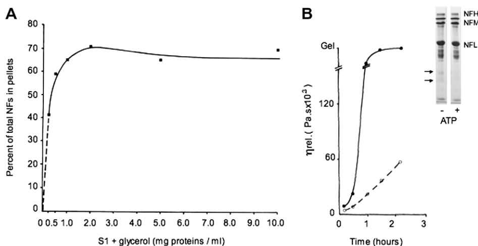
Fig. 1. ATP affects the yield and properties of purified NFs. (A) Increasing concentrations of the soluble extract of spinal cord in buffer A incubated with 4 M glycerol at 4 °C for 3 h (see Materials and methods) were centrifuged at 4 °C for 30 min at 176,000g (Airfuge Beckman). The relative fraction of sedimented NFs versus total NFs of the soluble extract (estimated by quantitative measurements of the triplet NFH + NFM + NFL by SDS-PAGE) is expressed as a function of the protein concentration of the extract in assays. (B) Viscosity kinetics of 3 mg/ml purified NFs obtained simultaneously from homogenates \pm 2 mM ATP. A strong gelation rate of NFs purified without ATP (filled circles and plain line) contrasts with that of NFs purified + 2 mM ATP (open circles and dotted line). Inset: 10% acrylamide SDS-PAGE of NFs purified without (-) or with (+) 2 mM ATP (40 \mu g loaded). Two minor proteins (arrows: apparent MW \approx 40 kDa and 30 kDa) regularly present in the purified NFs in the absence of ATP are released by ATP.
