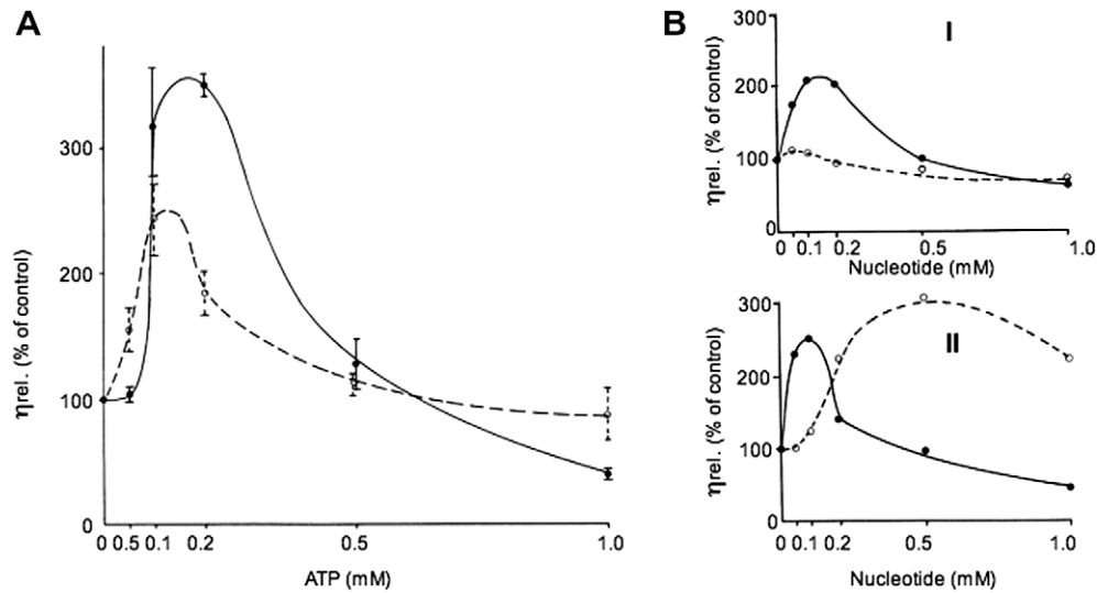
Fig. 4. ATP and AMP-PNP influence NF gelation in opposite concentration-dependent fashions. (A) Viscosity measurements of 4 mg/ml purified control (plain line, filled circles) and 0.8 M KCl-extracted NFs (dotted line, open circles) in the presence of increasing ATP (buffer B + 6 mM MgCl_2 ). Values after 2 h at 30 °C from three preparations are expressed as a % \pm SD of the viscosity of samples without ATP. (B) Comparison of the effect of increasing ATP (plain line, filled circles) and AMP-PNP (dotted line, open circles) on the viscosity of 3 mg/ml KCl-extracted (I) and control (II) NFs, after 2 h at 37 °C (buffer B + 6 mM MgCl_2 ). Values are expressed as a % of the viscosity of samples without nucleotide.
