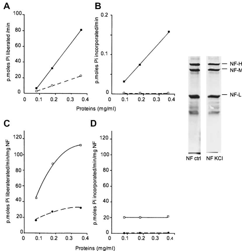
Fig. 2. The NF-associated ATPase activity is distinct from a couple kinase-phosphatase. Purified NFs (control and KCl-extracted) were analyzed at 35 °C for the hydrolysis of ATP and the phosphorylation of NF proteins in buffer B + 6 mM \text{MgCl}_2 . (A) ATPase activity (initial velocities of Pi release. NFs in buffer B + 6 mM \text{MgCl}_2 + 0.2 mM \gamma\text{-}^{32}\text{P} -ATP) measured for increasing concentrations of control (plain line and filled squares) and KCl-extracted (dotted line and open circles) NFs. (B) Incorporation of ^{32}\text{P} into proteins (in buffer B + 6 mM \text{MgCl}_2 + 0.05 mM \gamma\text{-}^{32}\text{P} -ATP) of increasing concentrations of control (plain line, filled squares) and KCl-extracted (dotted line and open circles) NFs. (C) Specific ATPase activities of control (plain line and open squares) and KCl-extracted (dotted line and filled circles) NFs from experiments of (A). (D) Specific autophosphorylation activity of control (plain line and open squares) and KCl-extracted NFs (dotted line and filled circles) from experiments of (B). Inset: Coomassie blue staining of control and KCl-extracted NFs analyzed on 10% SDS-PAGE (20 \mu\text{g} proteins loaded).
